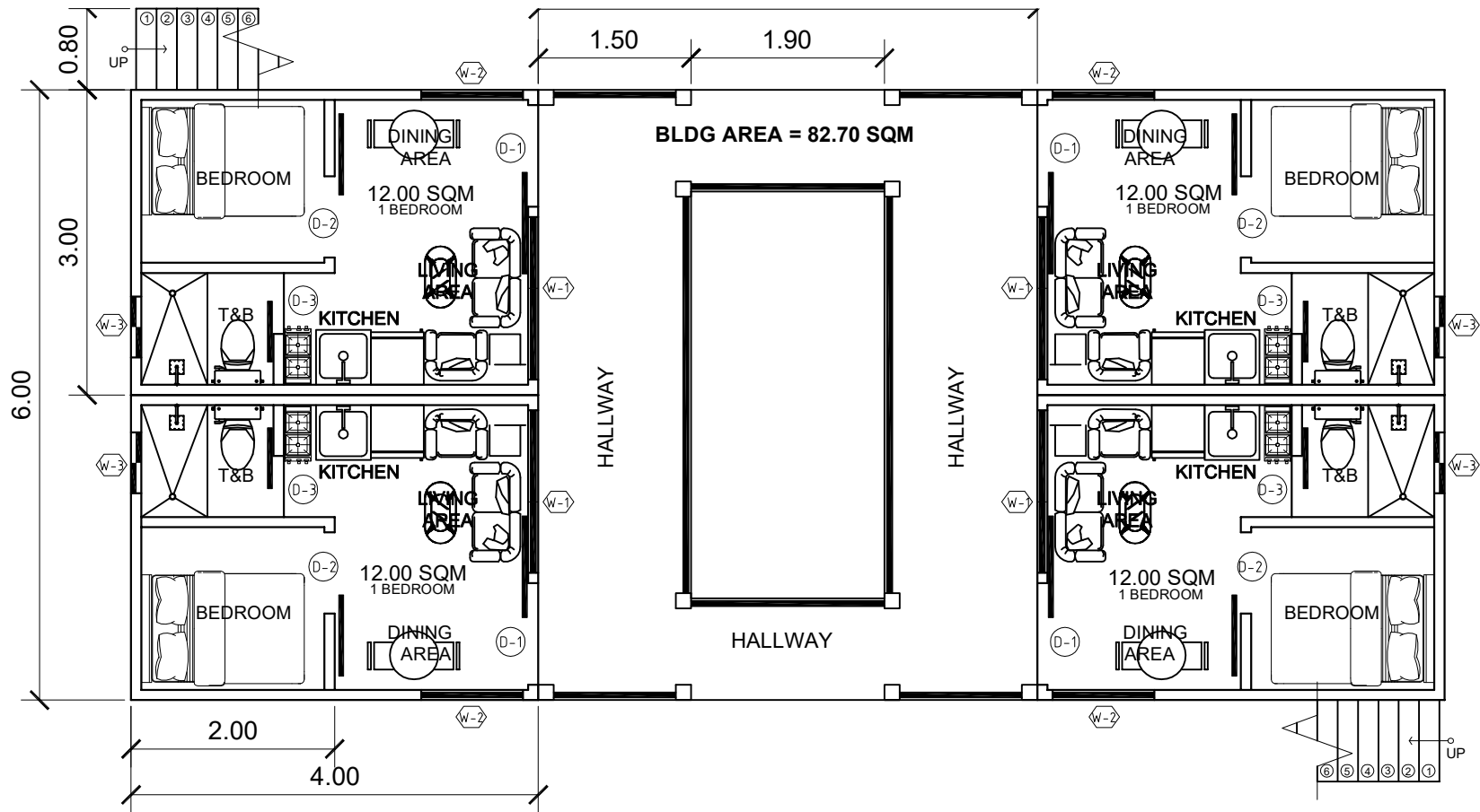
○ GROUND FLOOR PLAN SCALE 1:150
