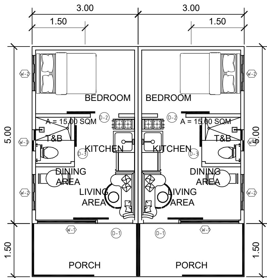
FLOOR PLAN SCALE 1:150
