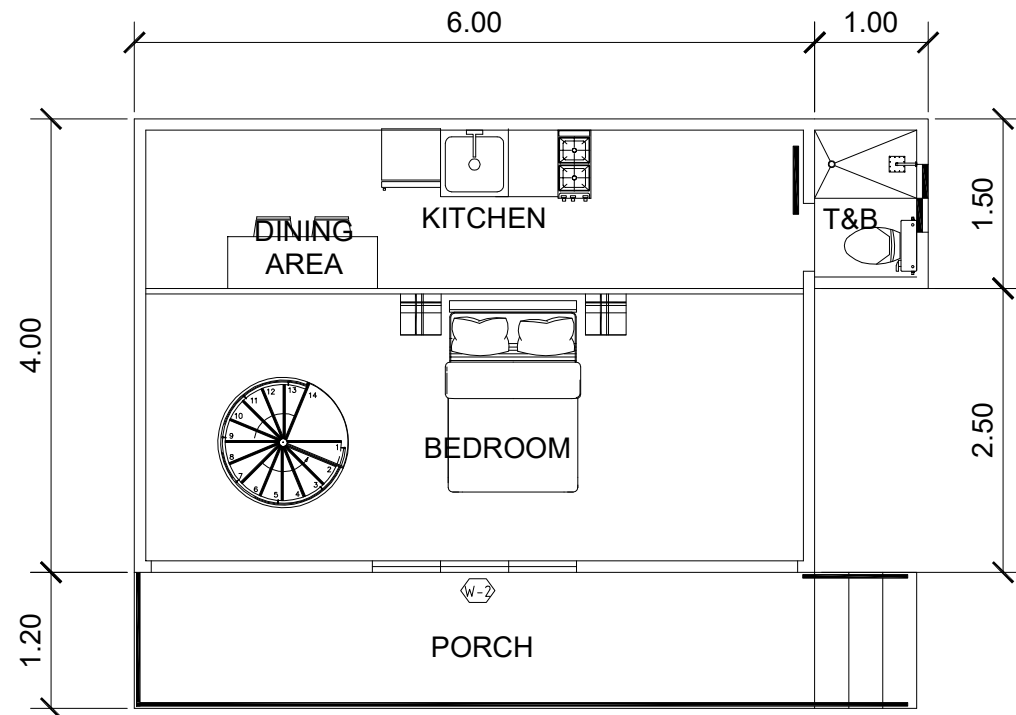
FLOOR PLAN SCALE 1:150
