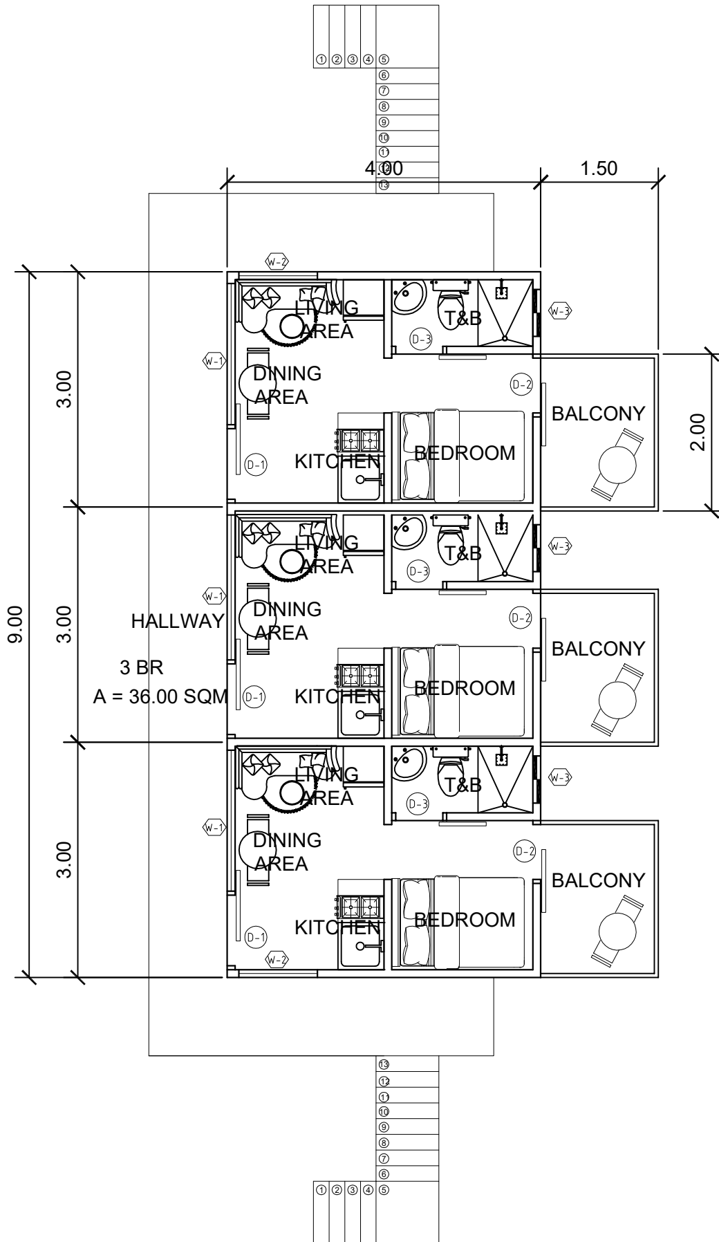
FLOOR PLAN SCALE 1:150
