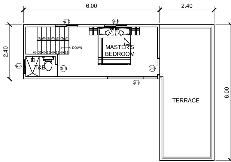
SECOND FLOOR PLAN SCALE 1:100
